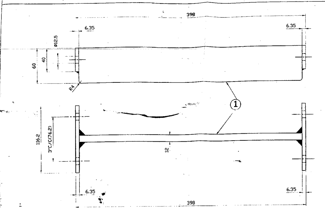
INSIDE LINK WITH SCRAPPER PLATE
