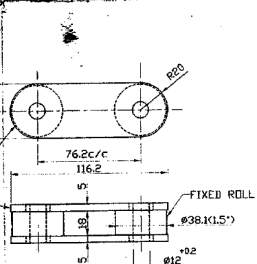
SIDE LINK WITH FIXED ROLL
